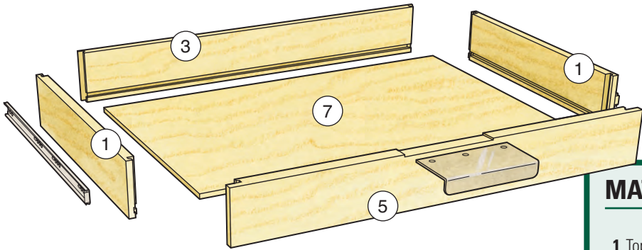
Exploded View
