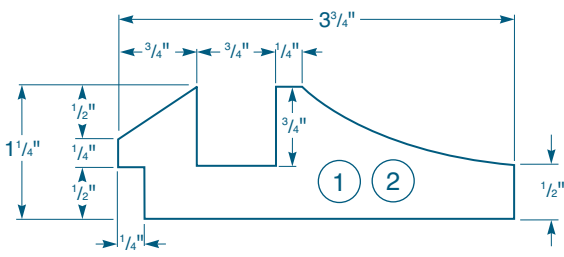
Frame Molding (Section View)
