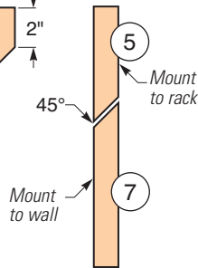
Cleats (End Views)
