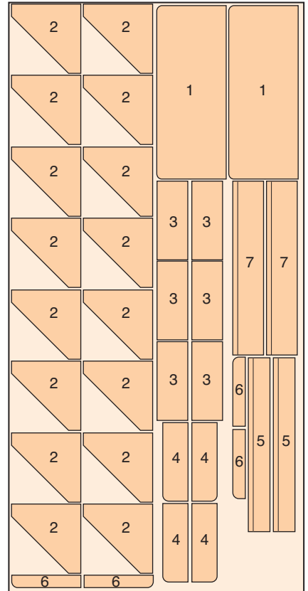
Cutting Diagram
